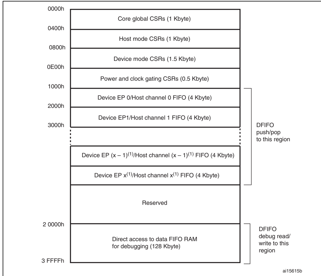
Figure 351. CSR memory map
