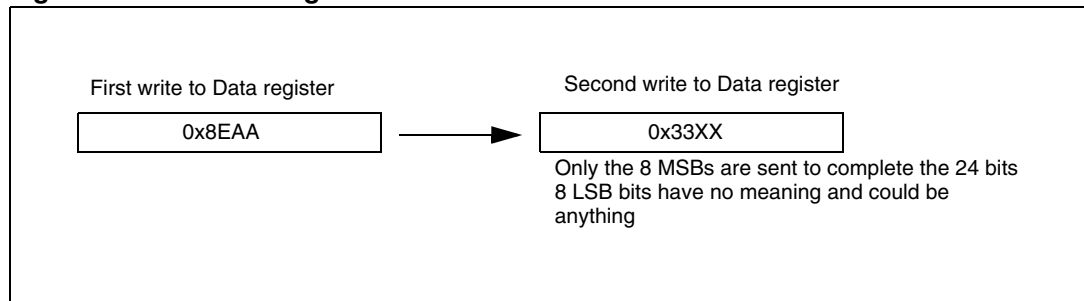
Figure 261. Transmitting 0x8EAA33
