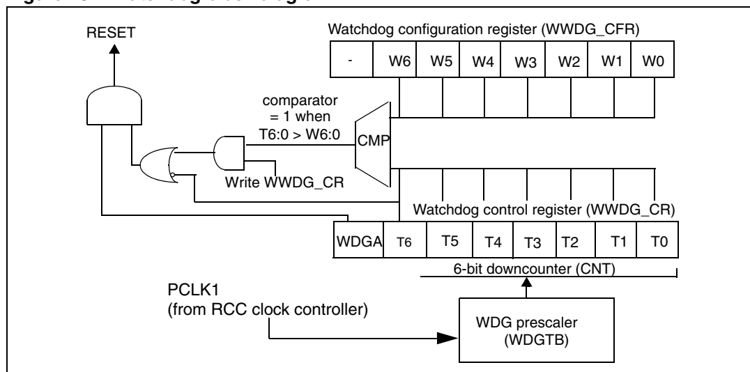
Figure 187. Watchdog block diagram
