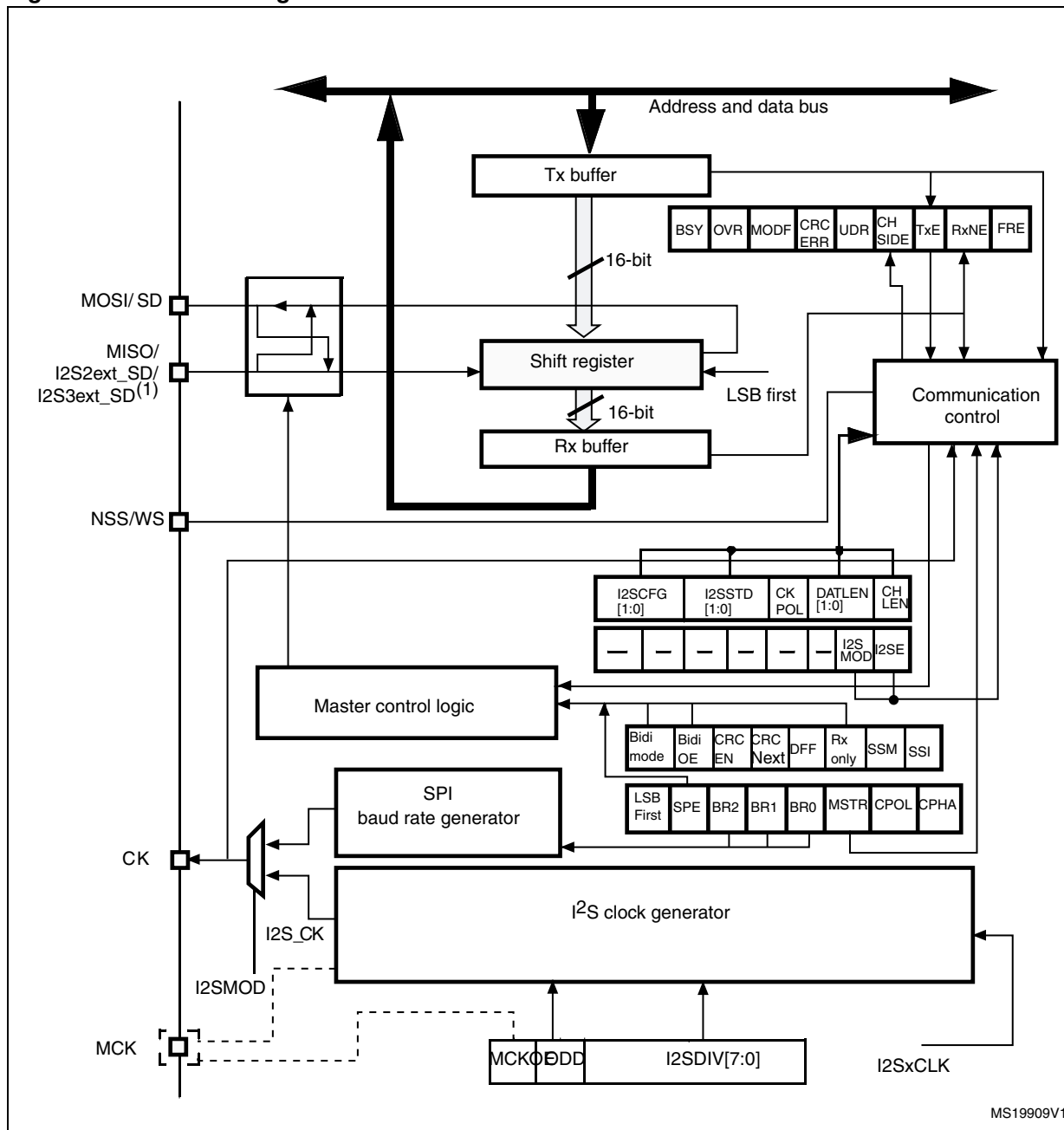
Figure 257. I 2 S block diagram
