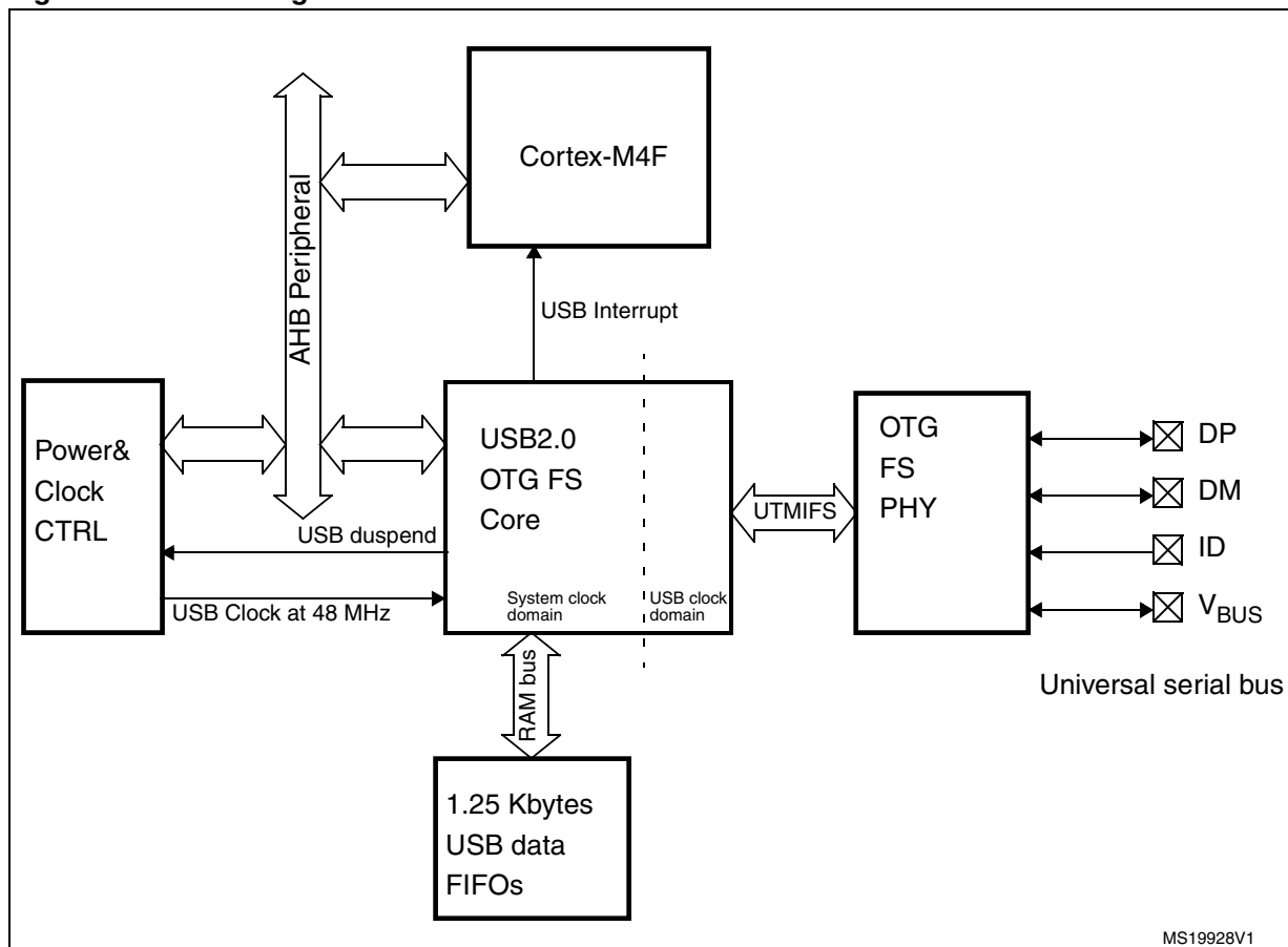
Figure 342. Block diagram
