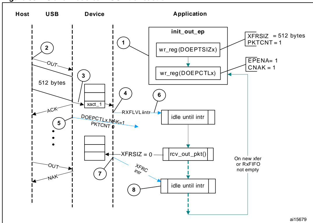
Figure 382. Slave mode bulk OUT transaction
