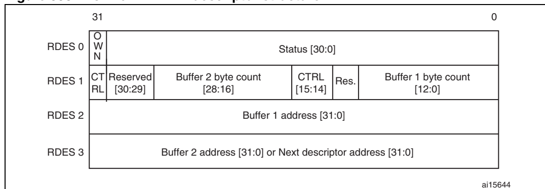
Figure 338. Normal Rx DMA descriptor structure
