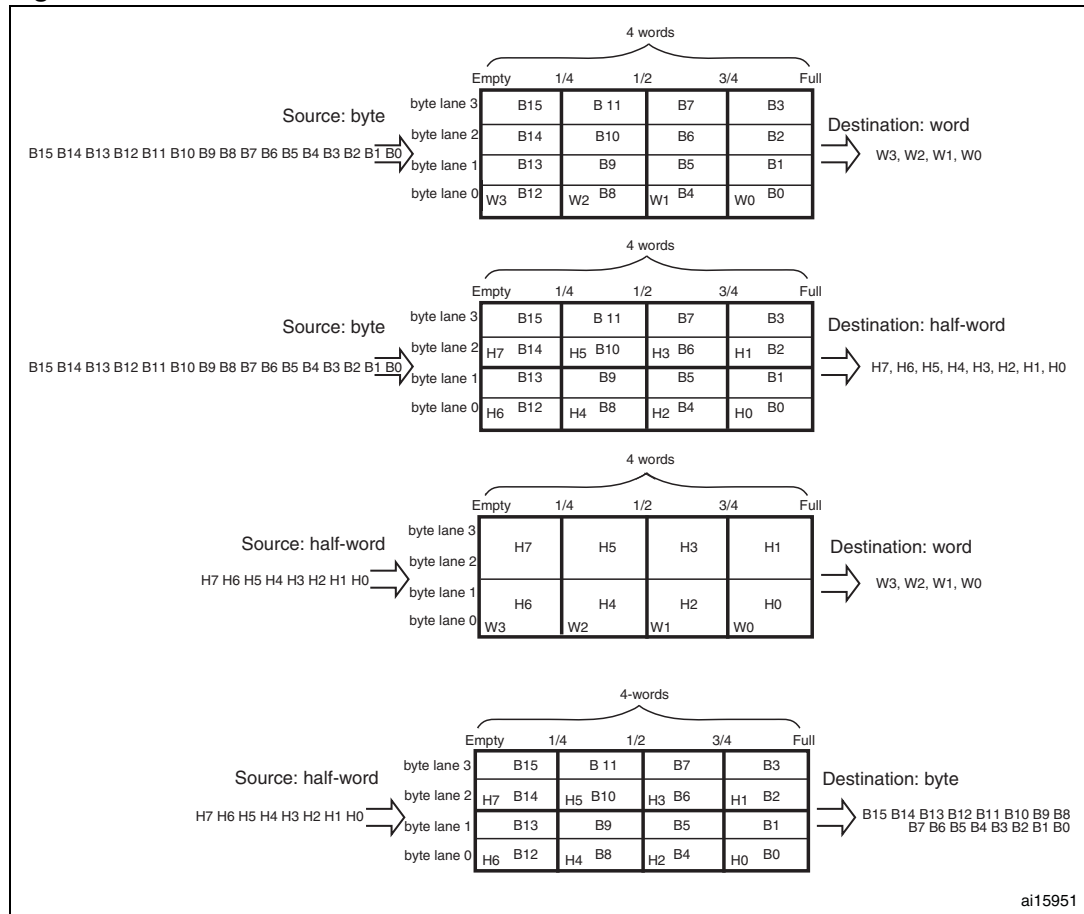
Figure 25. FIFO structure
