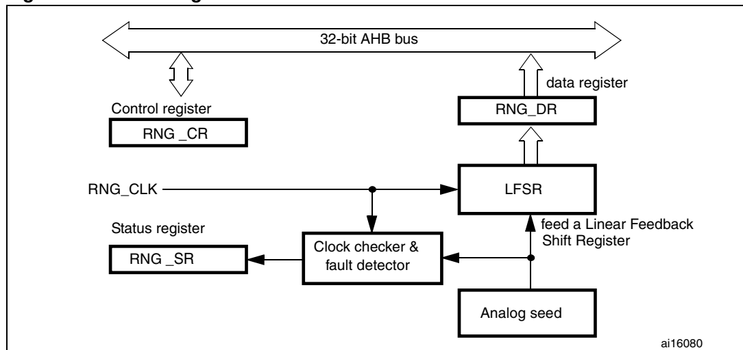
Figure 204. Block diagram
