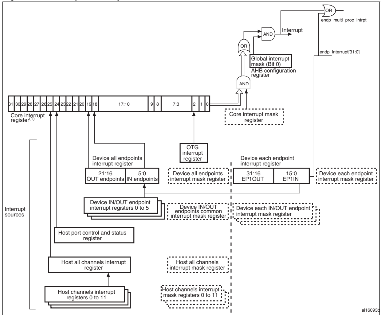
Figure 368. Interrupt hierarchy
