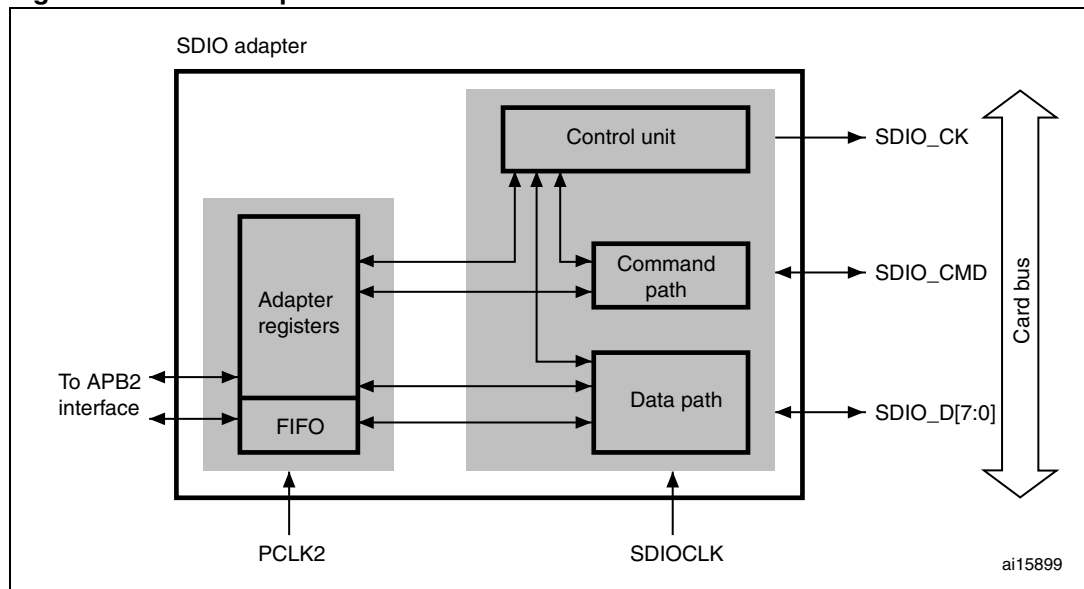
Figure 284. SDIO adapter
