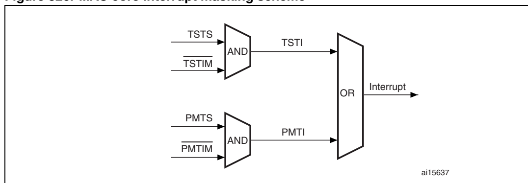
Figure 326. MAC core interrupt masking scheme
