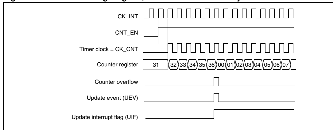
Figure 115. Counter timing diagram, internal clock divided by 1
