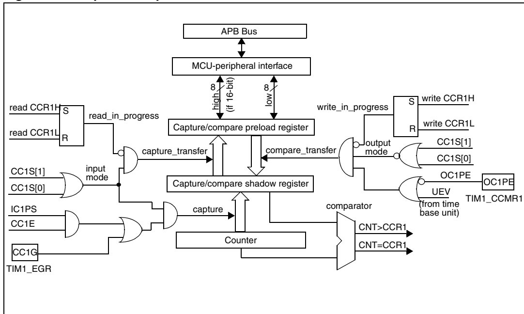
Figure 167. Capture/compare channel 1 main circuit
