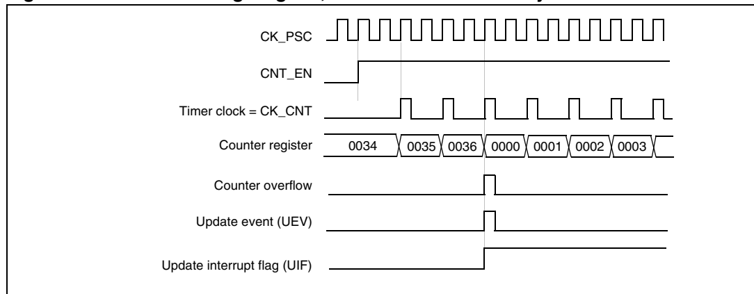
Figure 158. Counter timing diagram, internal clock divided by 2
