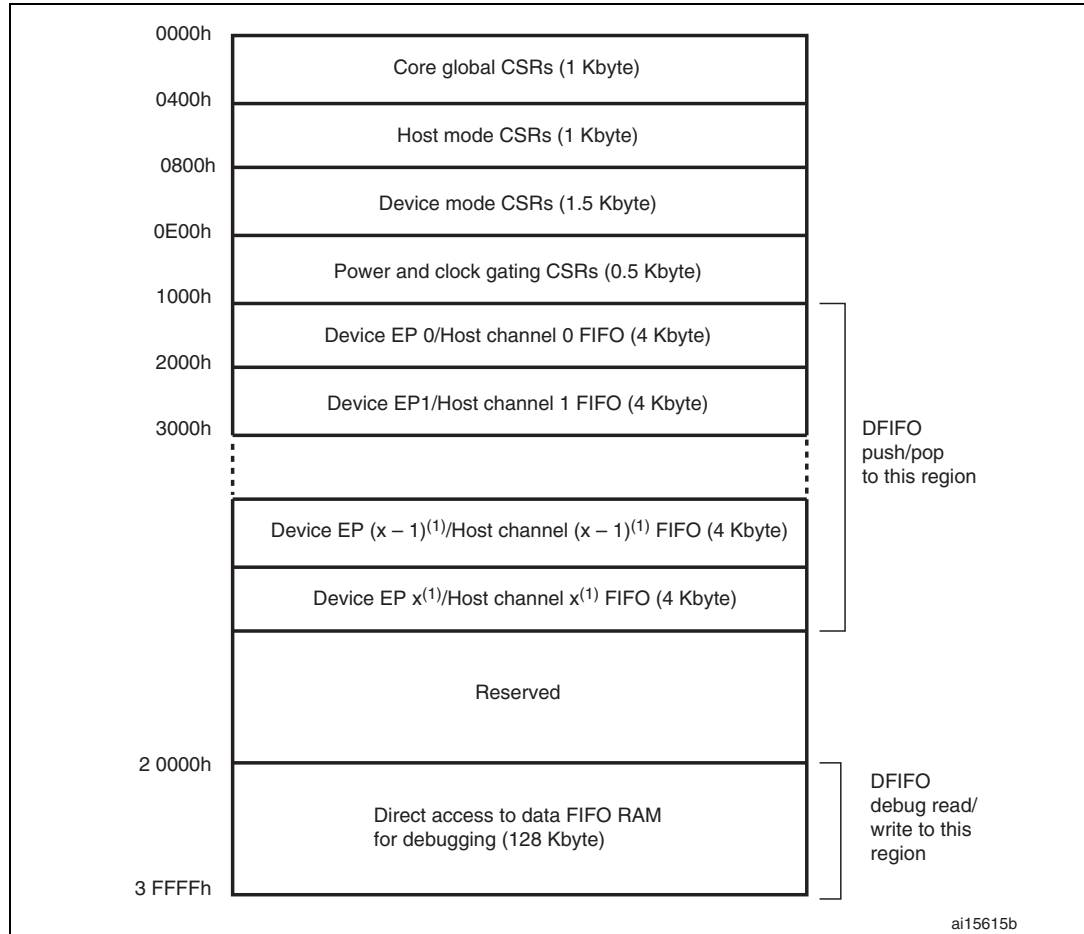
Figure 369. CSR memory map
