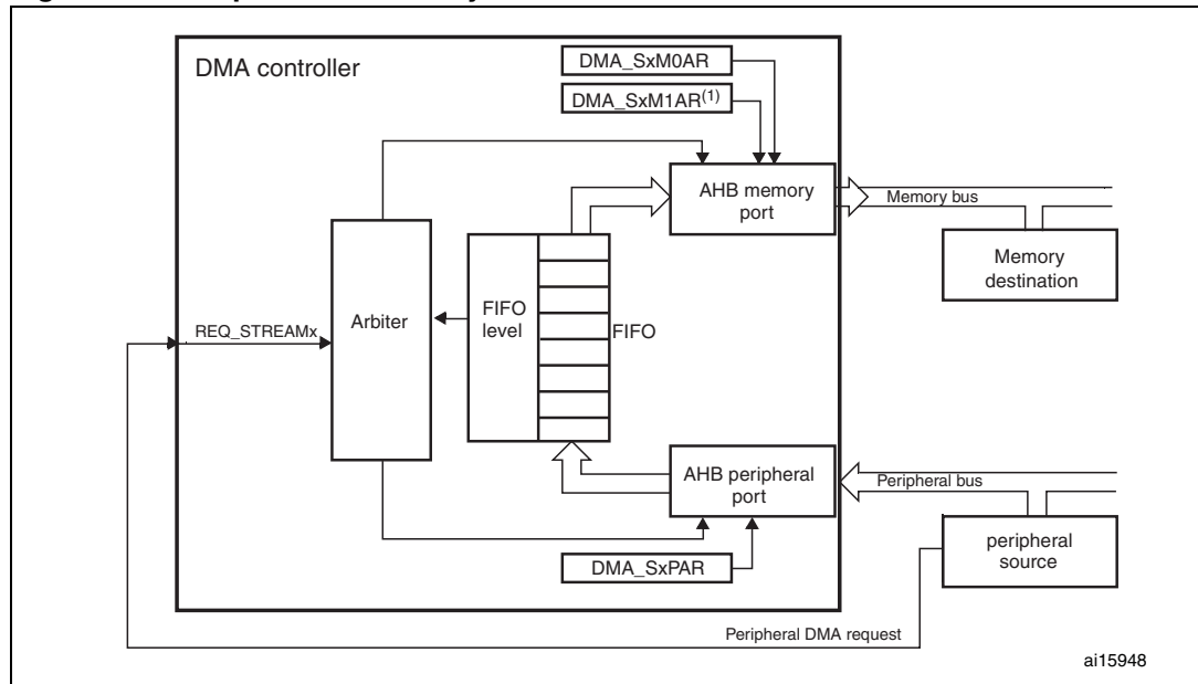
Figure 22. Peripheral-to-memory mode
