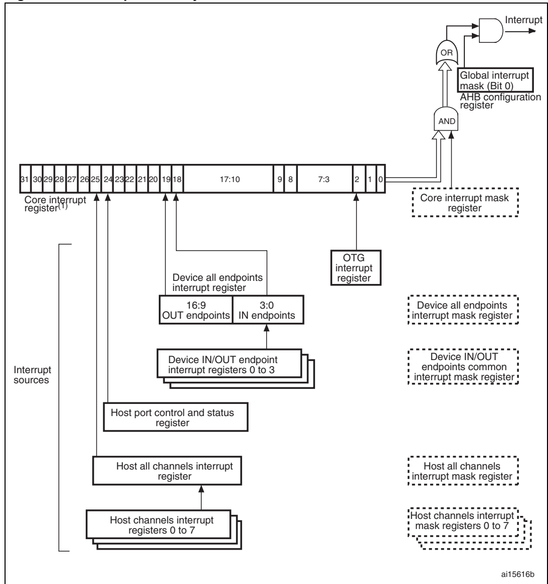
Figure 350. Interrupt hierarchy
