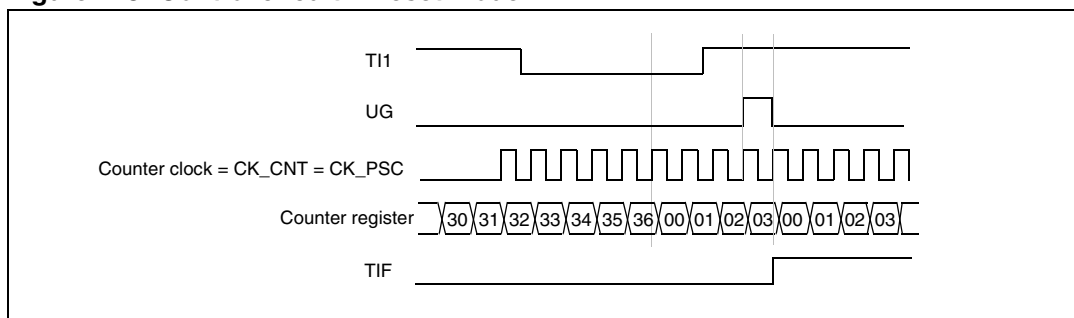
Figure 148. Control circuit in reset mode
