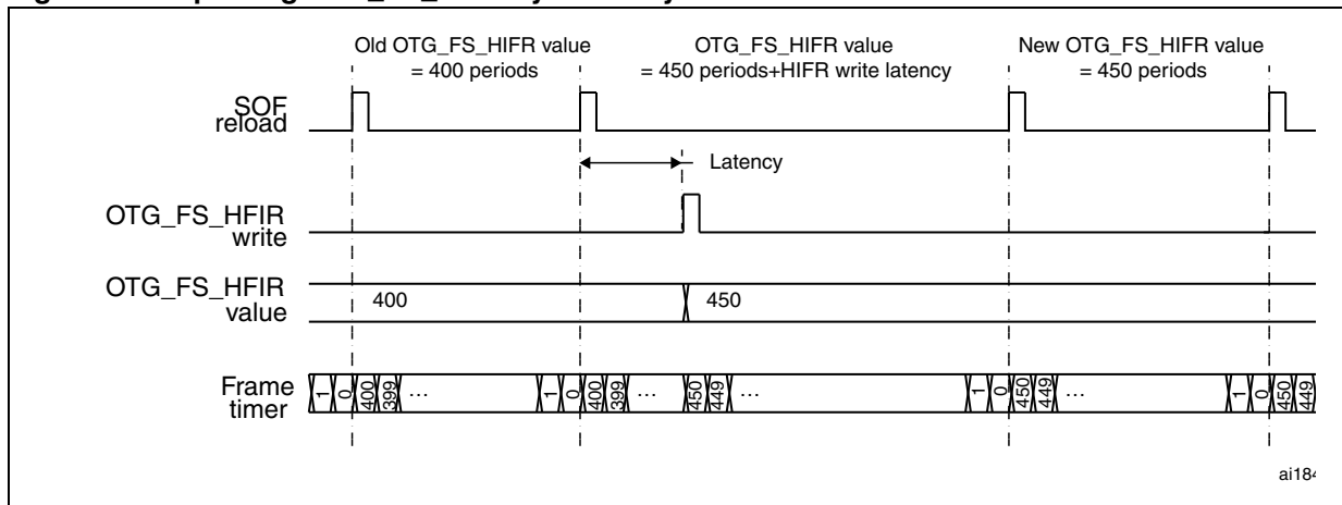
Figure 347. Updating OTG_FS_HFIR dynamically
