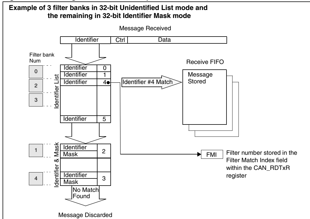
Figure 301. Filtering mechanism - example
