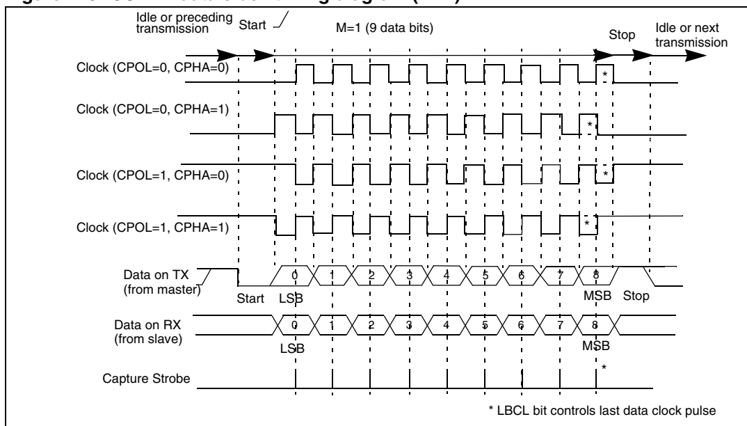
Figure 229. USART data clock timing diagram (M=1)
