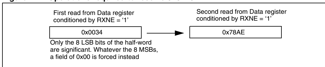
Figure 271. Operations required to receive 0x3478AE
