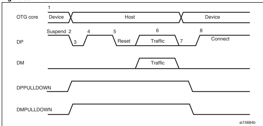
Figure 387. B-device HNP
