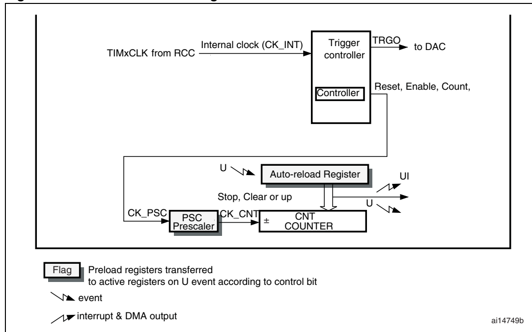
Figure 176. Basic timer block diagram
