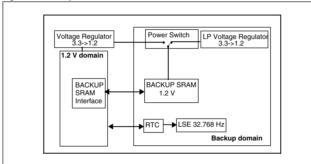
Figure 4. Backup domain
