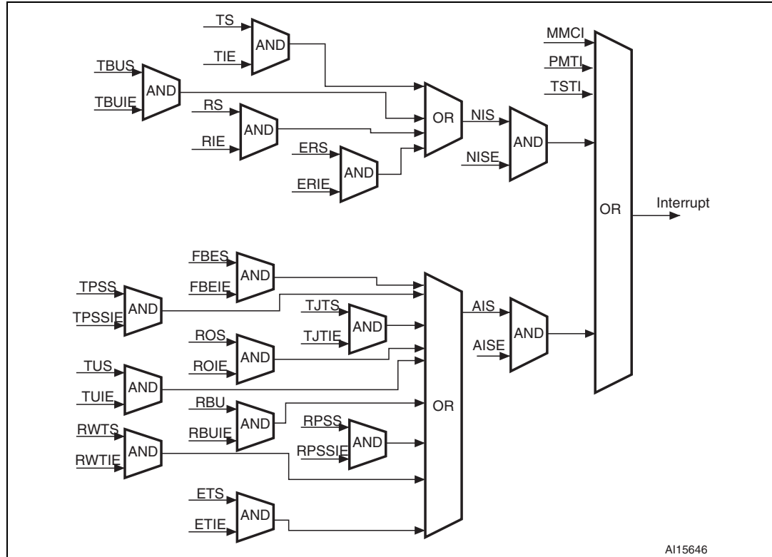
Figure 340. Interrupt scheme
