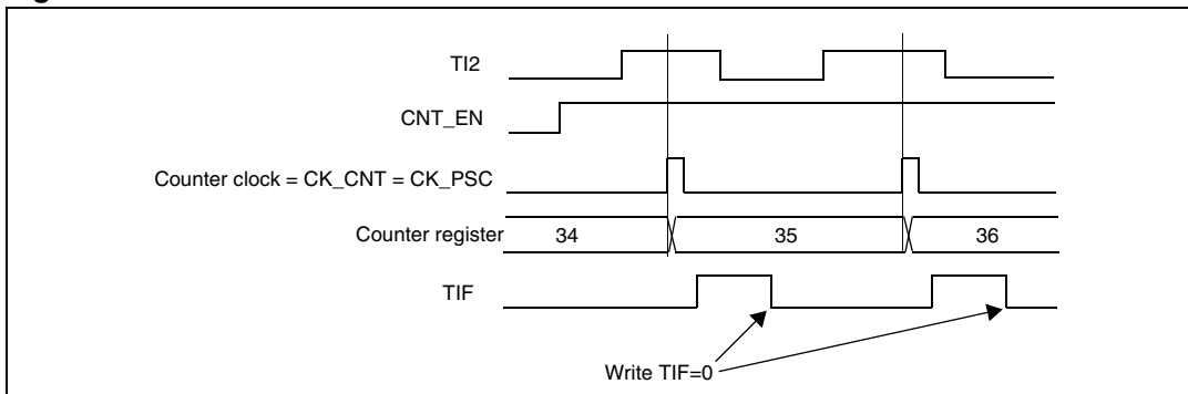
Figure 134. Control circuit in external clock mode 1
