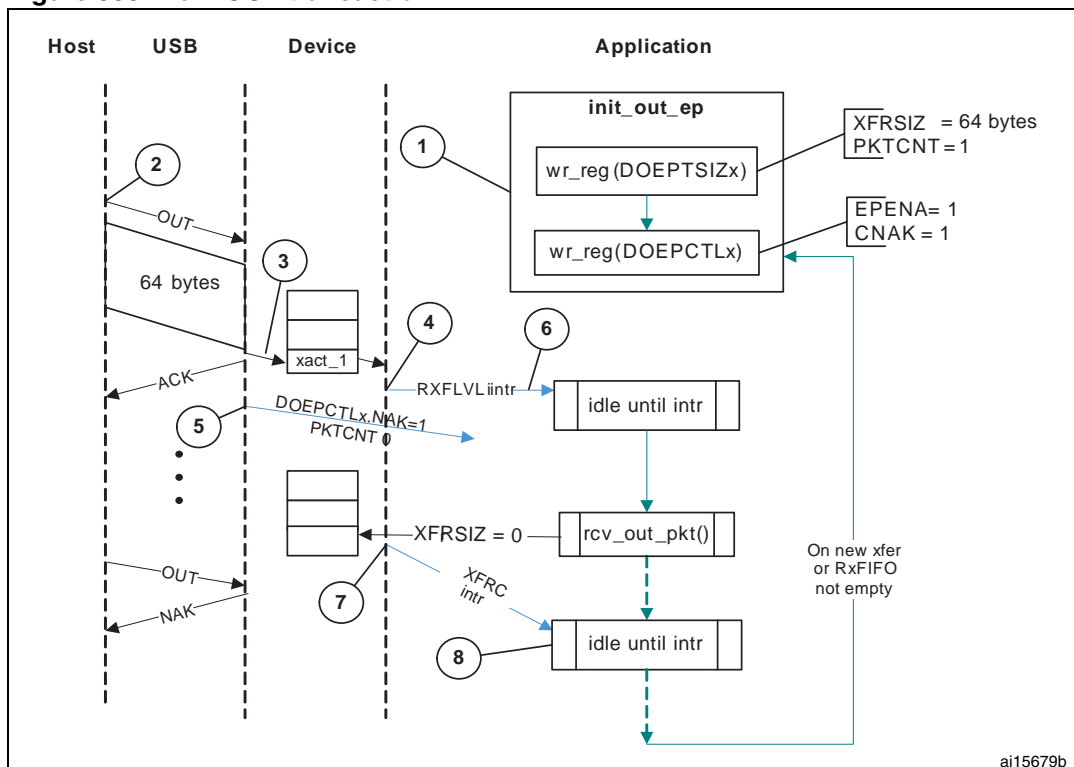
Figure 360. Bulk OUT transaction
