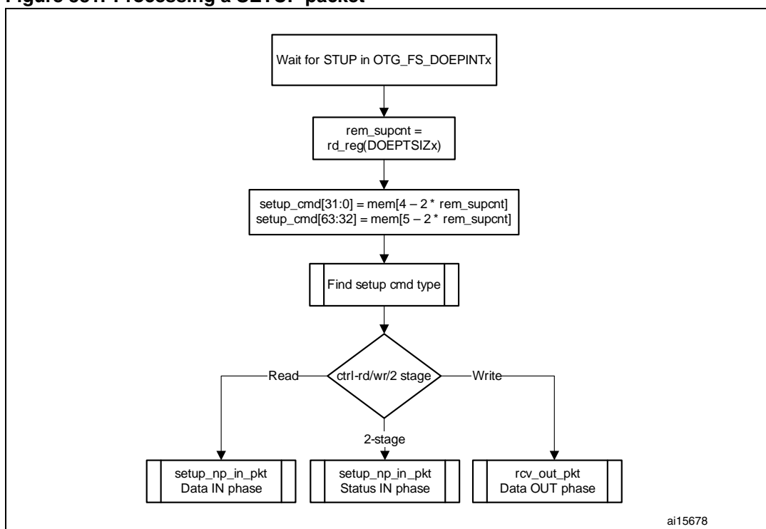
Figure 381. Processing a SETUP packet
