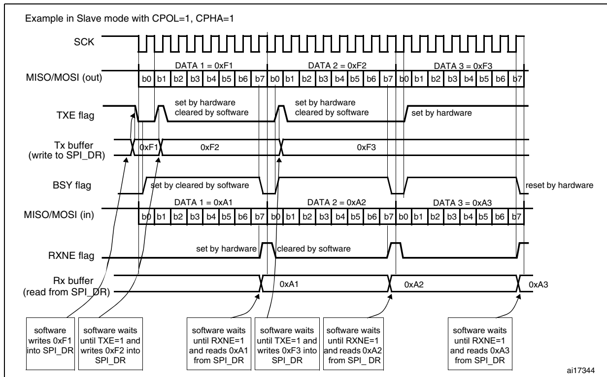
Figure 249. TXE/RXNE/BSY behavior in Slave / full-duplex mode (BIDIMODE=0, RXONLY=0) in the case of continuous transfers
