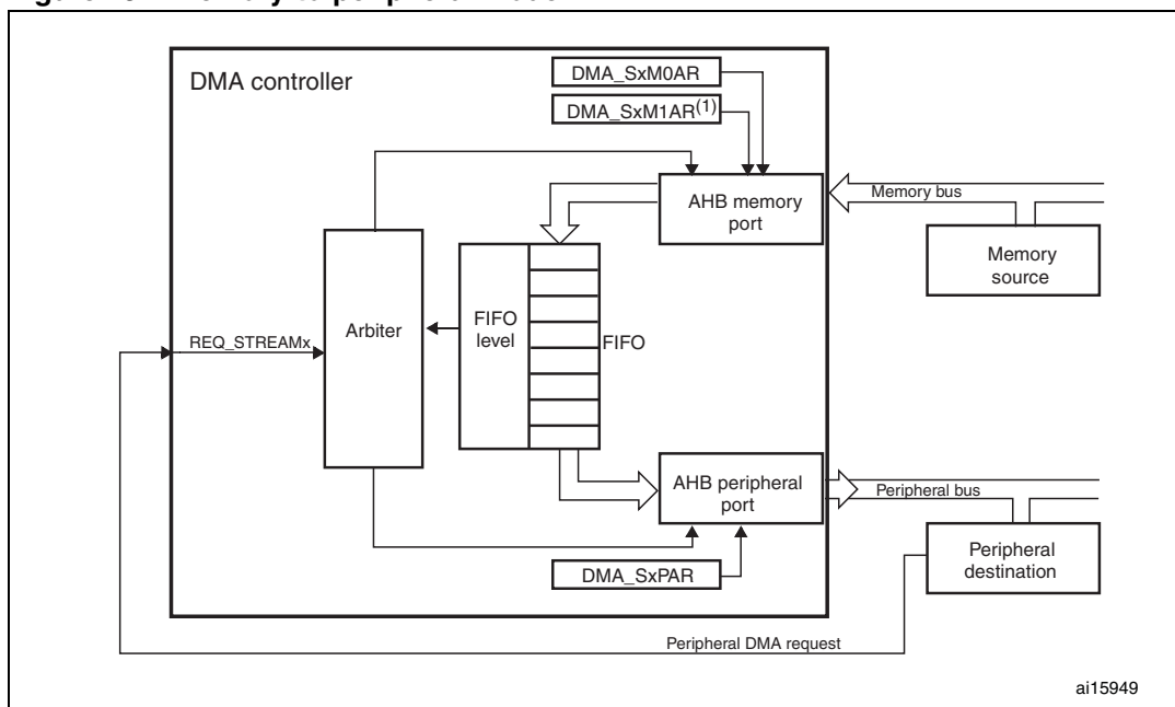
Figure 23. Memory-to-peripheral mode
