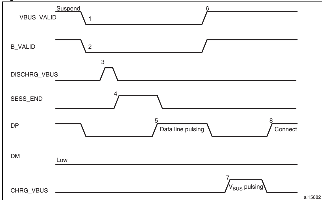
Figure 363. B-device SRP
