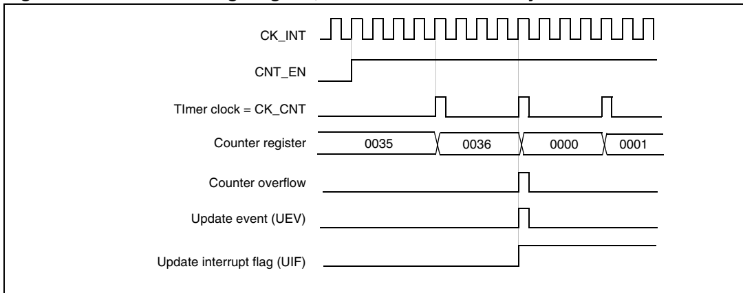
Figure 118. Counter timing diagram, internal clock divided by N
