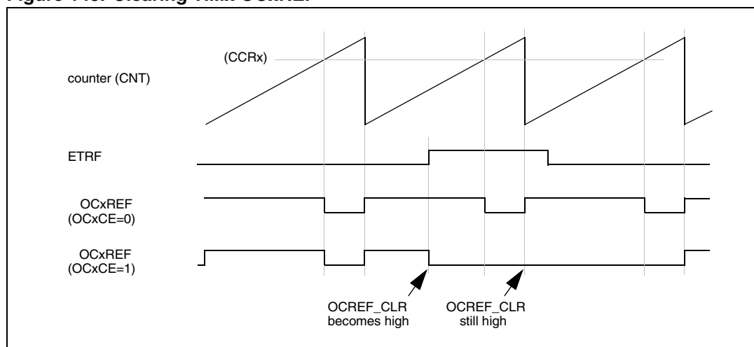
Figure 145. Clearing TIMx OCxREF
