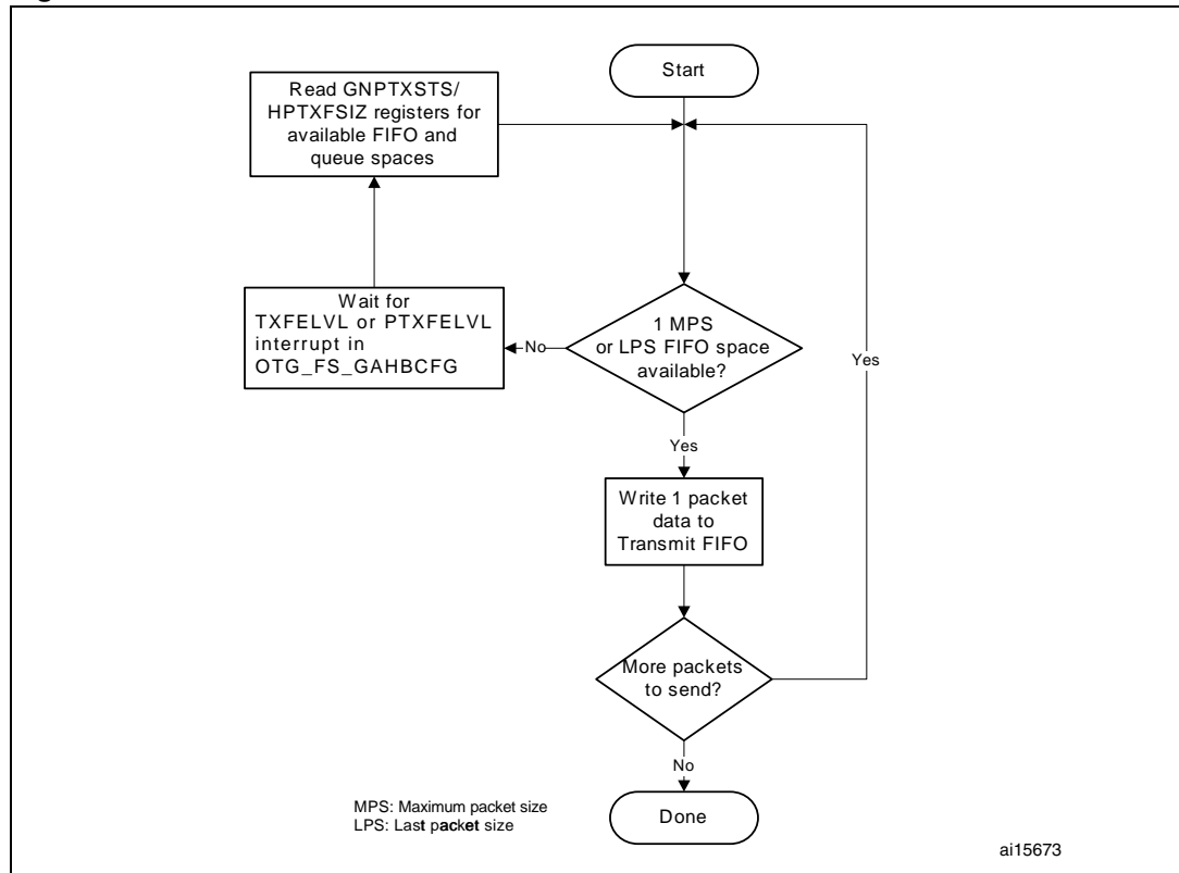
Figure 370. Transmit FIFO write task
