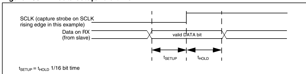
Figure 230. RX data setup/hold time
