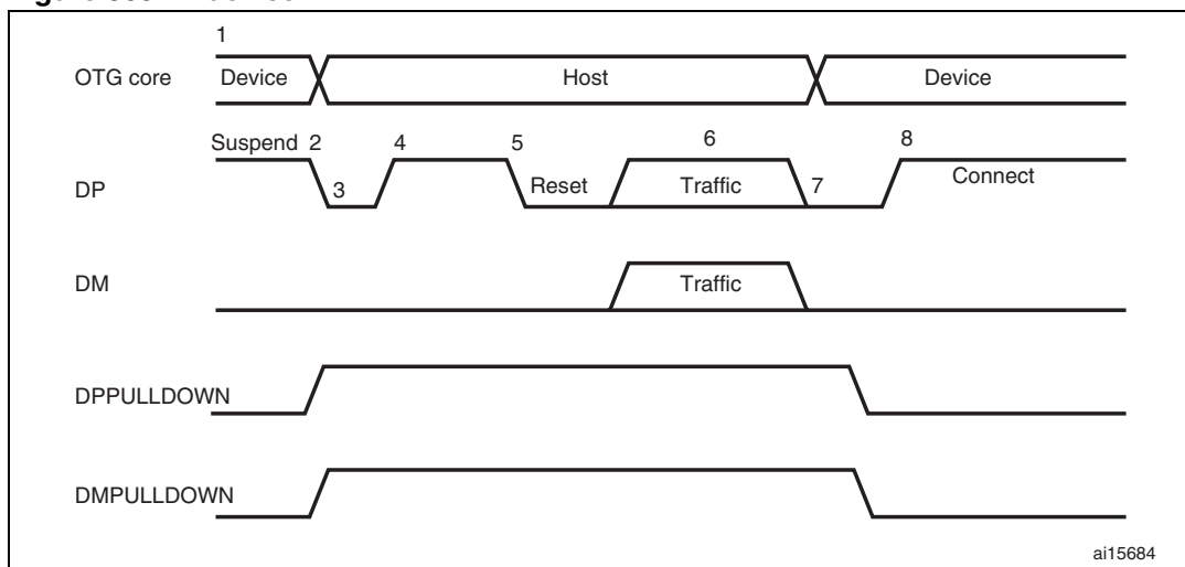
Figure 365. B-device HNP
