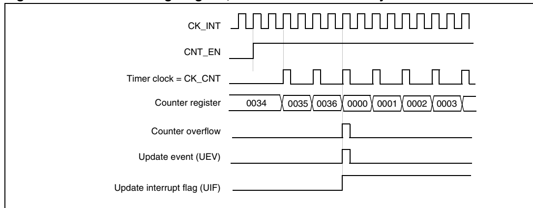
Figure 180. Counter timing diagram, internal clock divided by 2
