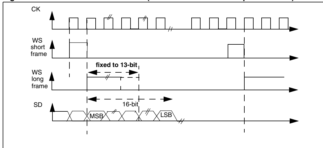
Figure 275. PCM standard waveforms (16-bit extended to 32-bit packet frame)
