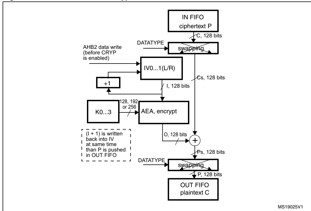
Figure 199. AES-CTR mode encryption
