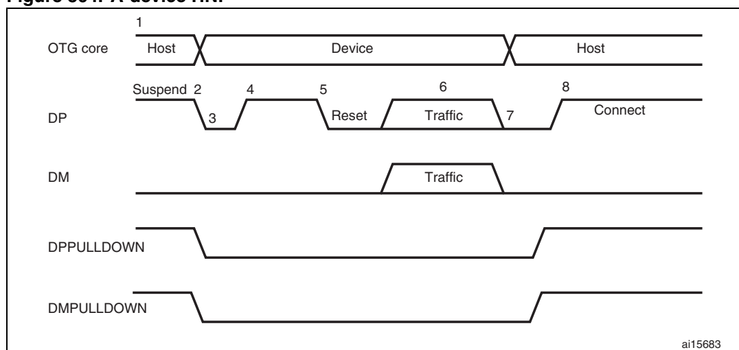
Figure 364. A-device HNP
