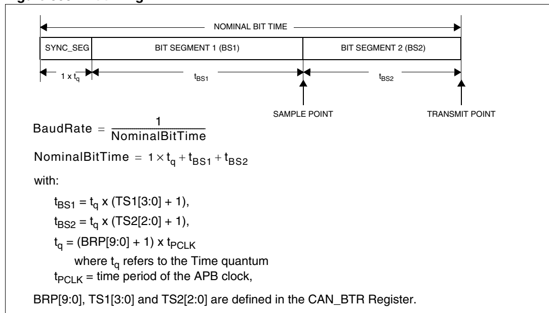
Figure 303. Bit timing
