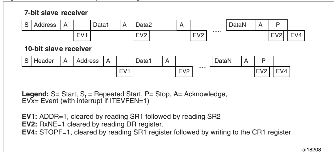
Figure 212. Transfer sequence diagram for slave receiver
