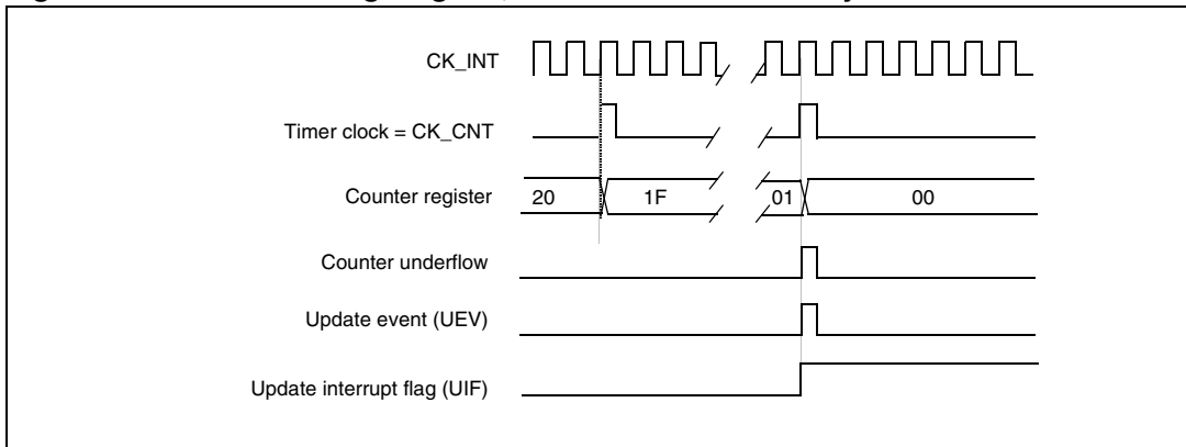
Figure 129. Counter timing diagram, internal clock divided by N
