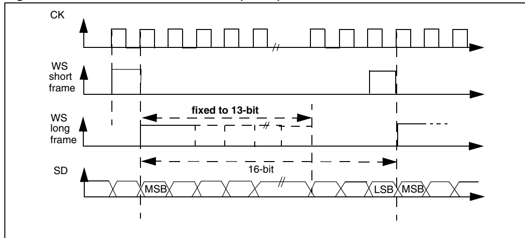
Figure 274. PCM standard waveforms (16-bit)
