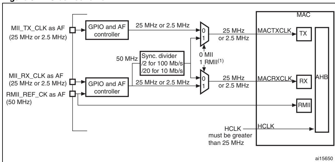
Figure 314. Clock scheme
