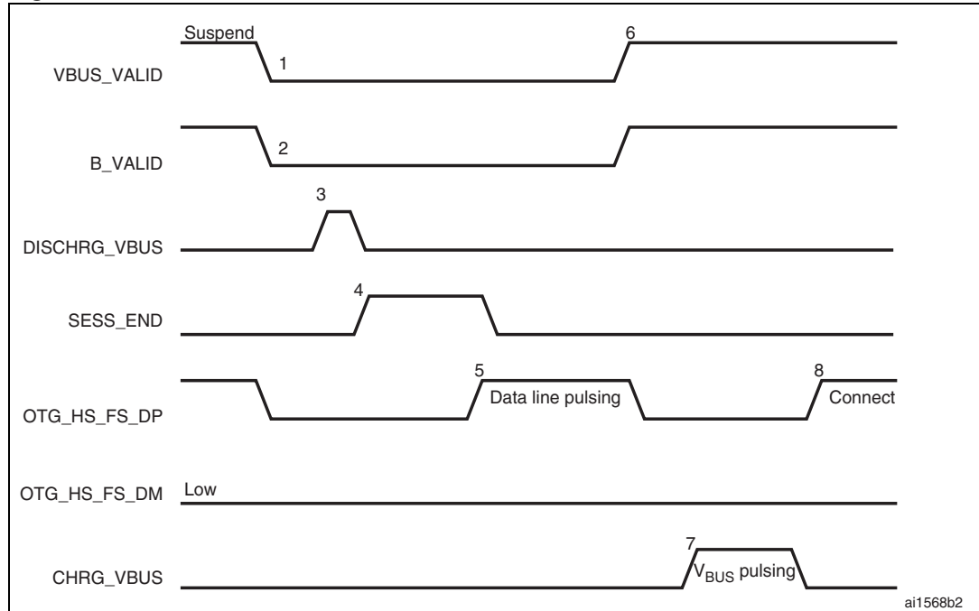
Figure 385. B-device SRP
