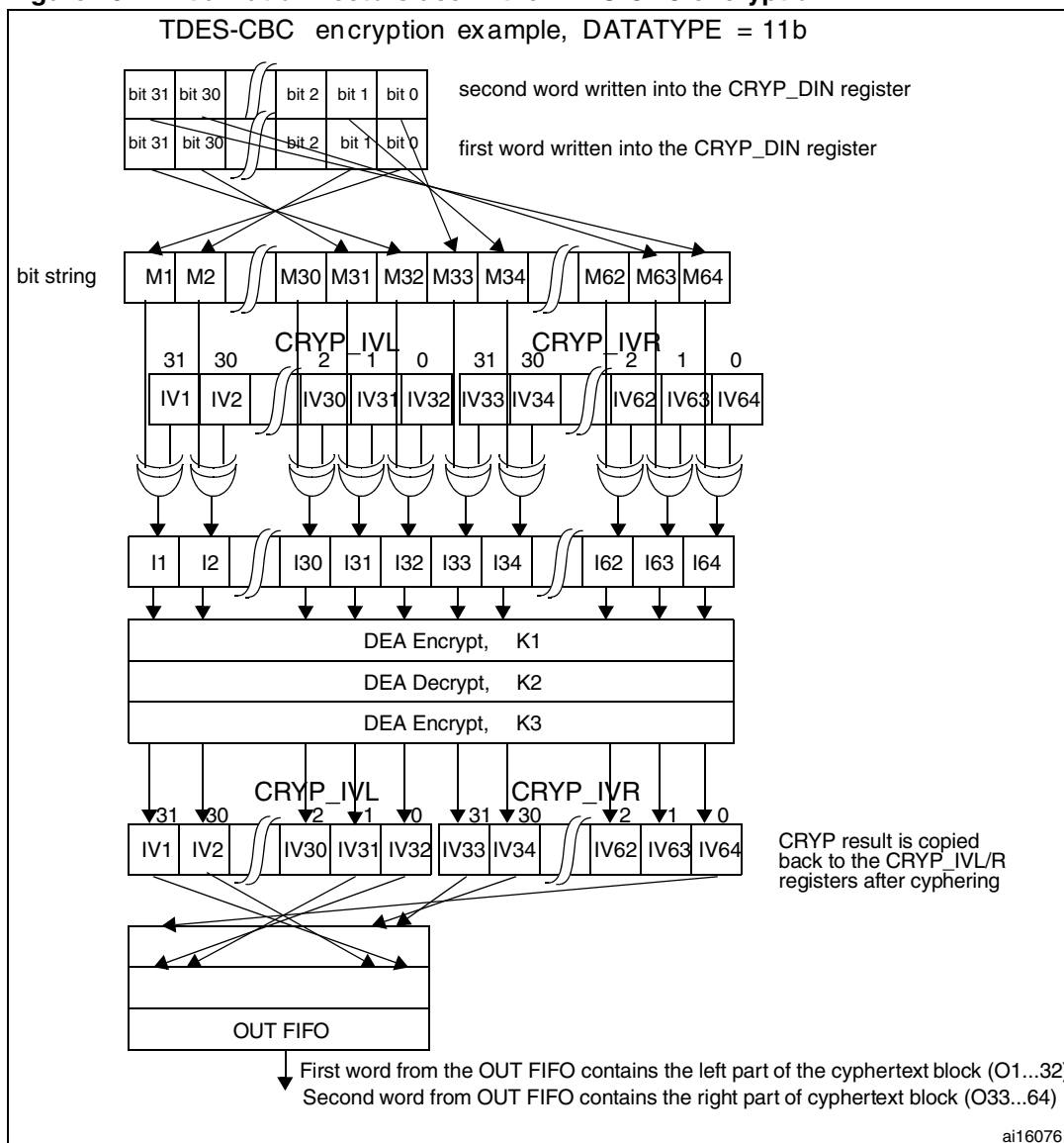
Figure 202. Initialization vectors use in the TDES-CBC encryption
